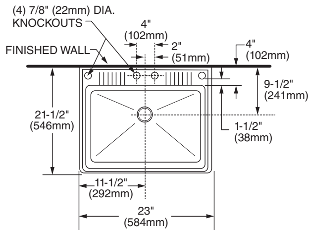
MODEL L-1 WALL HUNG
